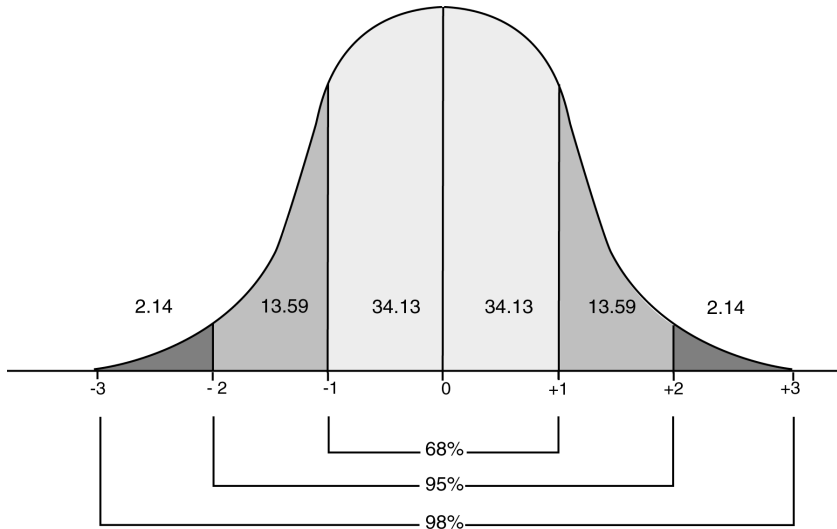
Figure 1.1: Normal Distribution
